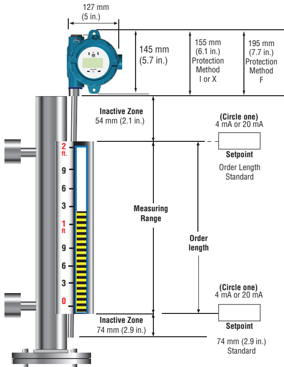
Figure 2. CHAMBERED mounting, bottom flange *
