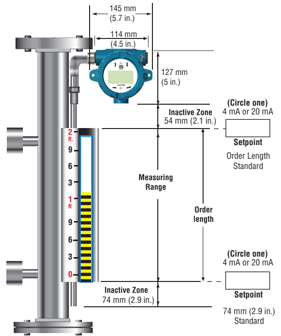
Figure 3. CHAMBERED mounting, top and bottom flange *
